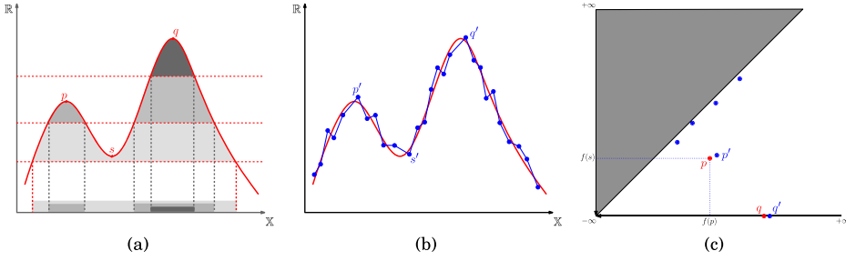
Fig. 1. Sketch of topological persistence: (a) a new connected component is born in the superlevel-set F^\alpha when \alpha = f(p) , and it dies when \alpha = f(s) ; its lifespan is represented as a point in the PD of f ; (b) a piecewise-linear approximation \tilde{f} of f ; (c) superimposition of the PDs of f (red) and \tilde{f} (blue), showing the one-to-one correspondence between the prominent peaks of f and \tilde{f} .
