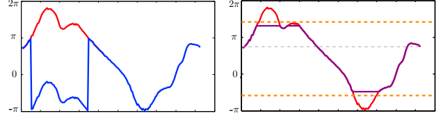
Figure 10: SyntheticC. Left: The phase plot, original version (blue), and the phase-unwrapped version (red). Right: The phase plot with optimal unwrap point (orange) and the modified phase plot with boundary uncovered (purple).
