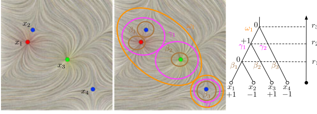
Fig. 2. Figure from [29] showing the merge tree for a 2D vector field example. The robustness computation and merge tree construction are the same in all dimensions. Suppose the vector field is continuous, where sinks are red, sources are green, and saddles are blue. From left to right: vector field f , relations among components of \mathbb{F}_r , and the augmented merge tree. f contains four critical points: a sink x_1 , a source x_3 , and two saddles x_2 and x_4 . We use \beta , \gamma , \omega , etc. to represent components of the sublevel sets.
