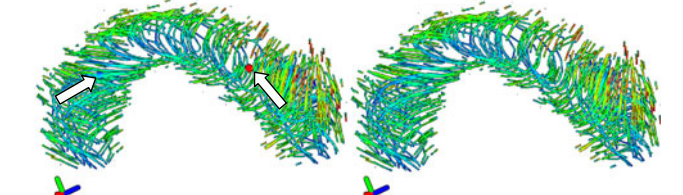
Fig. 11. DeltaWing#1 before (left) and after (right) simplification. Critical points to be simplified are indicated by arrows.
