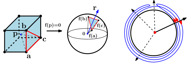
Fig. 3. Left: mapping between tetrahedra (a, b, c, p) and (f(a), f(b), f(c), O) . Right: computing the winding number of a curve, where \text{winding\#} = \text{\#up-crossings} - \text{\#down-crossings} = 2 - 1 = 1 .
