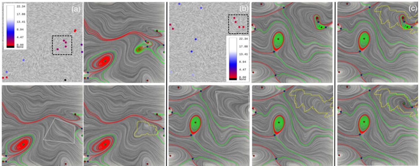
Fig. 12. The OceanA dataset: (a) #20311; (b)-(c) #21217. (a)-(b) For each subfigure, Top Row: Left—shows robustness values with region of interest highlighted; Right—shows the vector field marked by critical point types and its topological skeleton. Bottom Row: results after distance-based (left) and robustness-based simplifications (right). (c) A region (yellow boundary) with a nontrivial Conley index and uncovered boundary (top), where smoothing does not remove its critical points (bottom).
