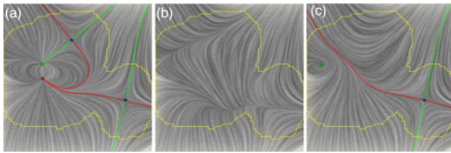
Fig. 7. SyntheticB. (a) the original vector field with its topological skeleton. (a)-(b): Single level simplification before (a) and after (b) by Cut and Smoothing. (c) Only applying Smoothing does not make the region a critical point free field.
