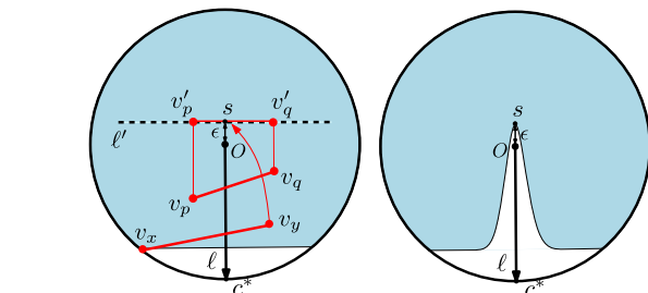
Fig. 5. Cut operation. Left: The projection of edges that intersect \ell during the Cut operation. Right: After Cut , the light blue region represents \text{im}(C) , which no longer contains (covers) the origin and so is critical point free.
