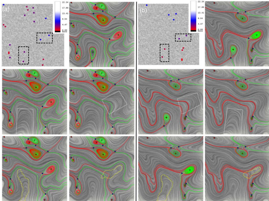
Fig. 11. (a) The OceanB dataset. (b) The OceanC dataset. For each subfigure: Top Row: Left—shows robustness values with the region of interest highlighted (robustness values are colored from red to white, where red means low and white means high robustness); Right—shows the vector field marked by critical point types along with separatrices. Middle Row: the two-step hierarchical simplification based on distance. Bottom Row: the two-step hierarchical simplification based on robustness.
