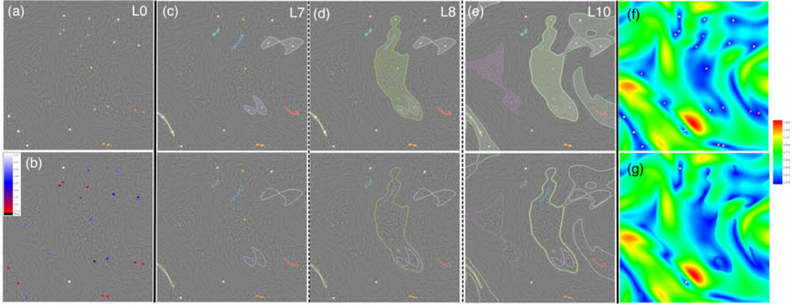
Fig. 17. Hierarchical simplification of CombustionB . (a)-(b): Vector field before simplification where critical points are colored by robustness pairing (a) and robustness values (b). (c)-(e): Different levels of simplification, levels 7, 8 and 10, with robustness values 0.29, 0.35 and 0.39, respectively; vector fields before (top row) and after (bottom row) simplification. (f)-(g) Vector field magnitude functions before (f) and after (g) simplification.
