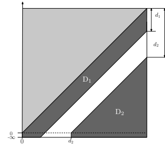
Figure 3: Separation of the persistence diagram D_0 f between prominent peaks ( D_2 ) and topological noise ( D_1 ).
